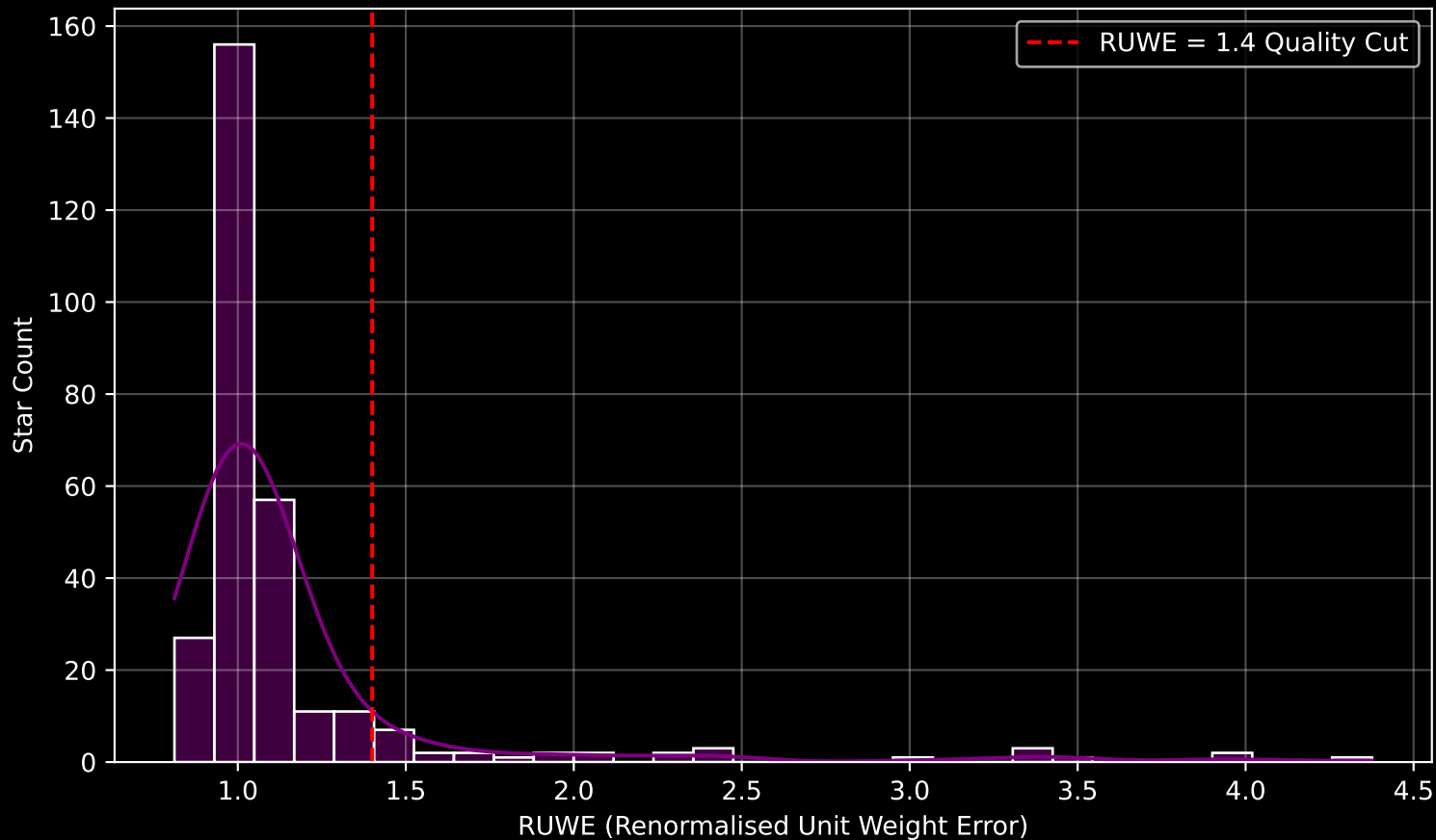
GALAH DR4 Field [-4] RUWE Distribution (n= 291)
