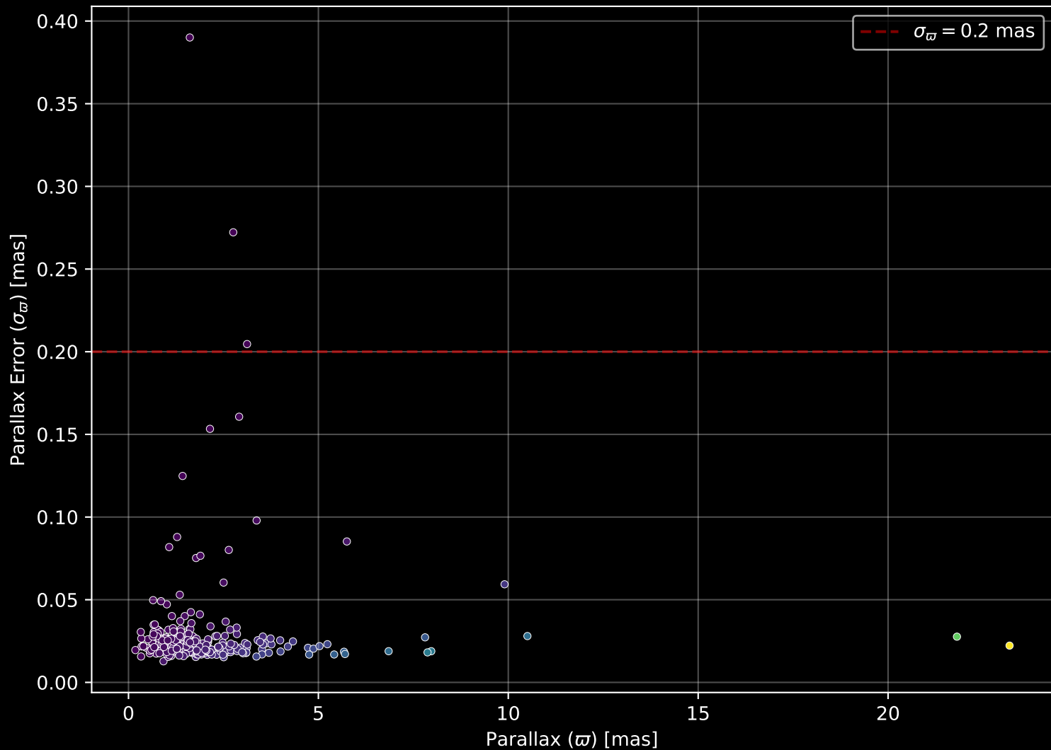
GALAH DR4 Field: [-4] Parallax Quality (n= 298)
