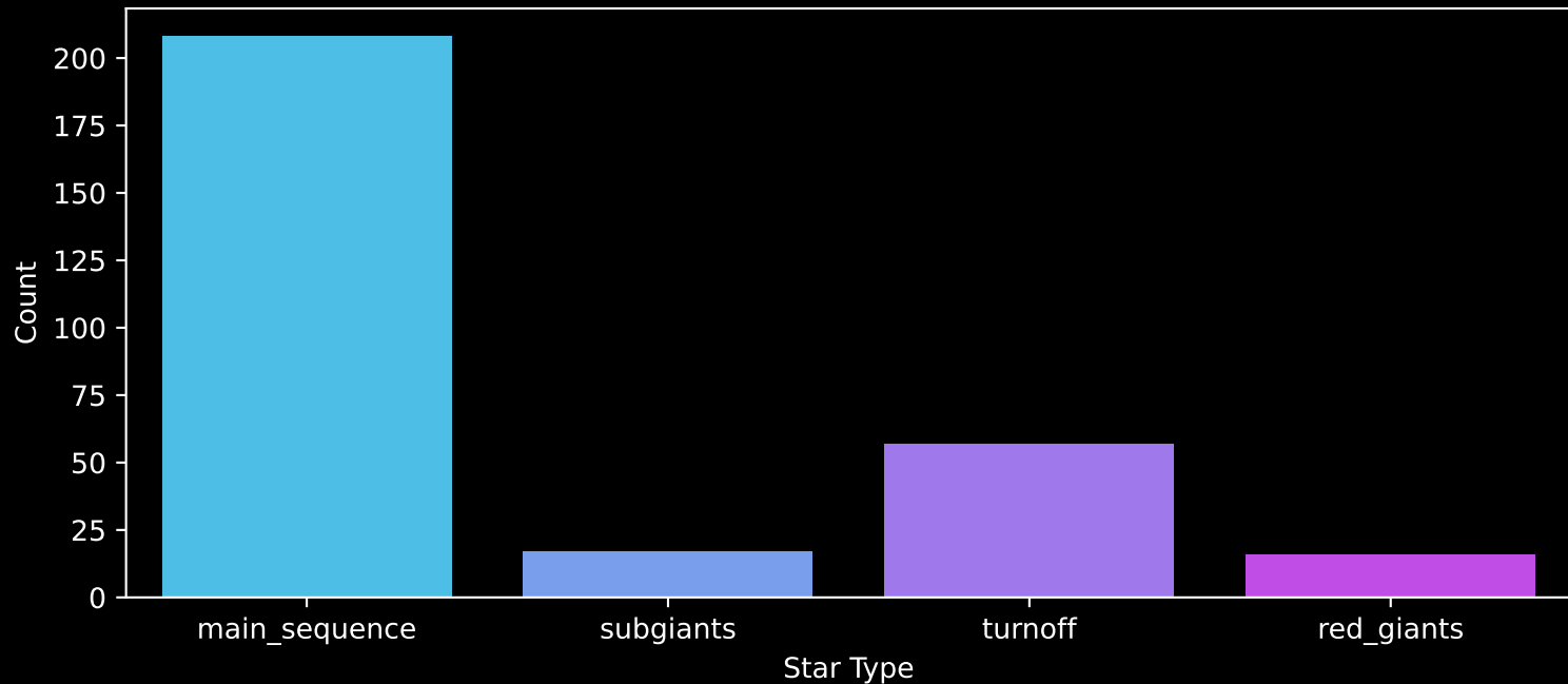
GALAH DR4 Field: [-4] Count plot of Star Type
